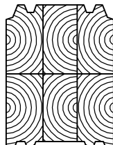
Sharpline-profile
